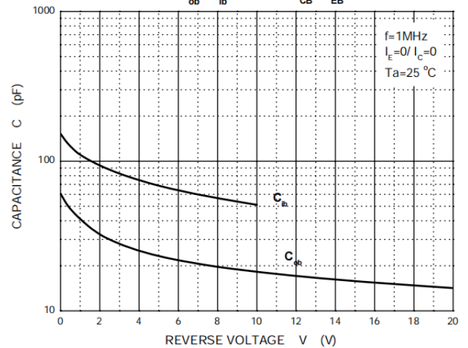
C_{ob}/C_{ib} — V_{CB}/V_{EB}
