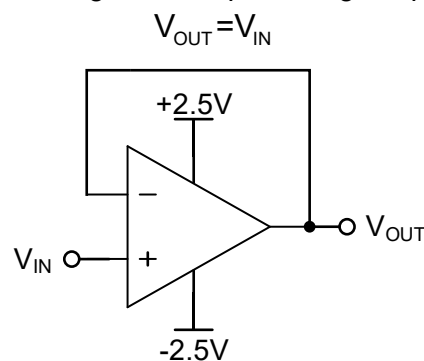
Figure 12. Voltage Follower
