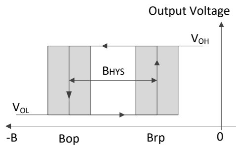
TO-92S/SOT-23
