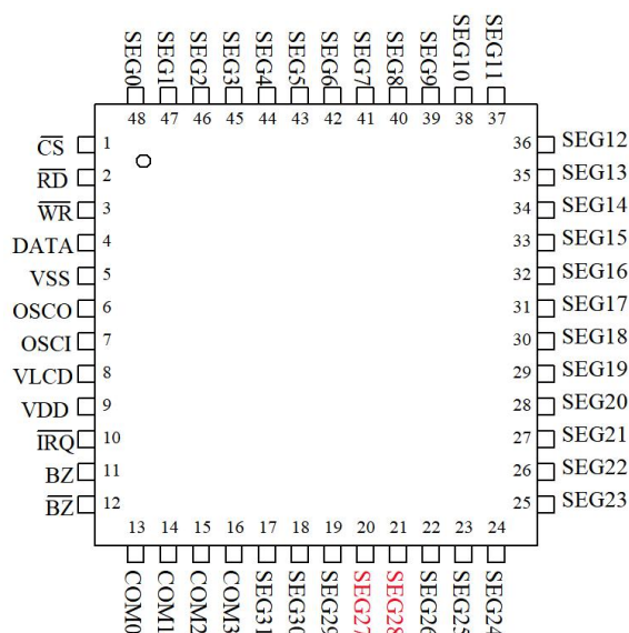
TM1621B LQFP-48
