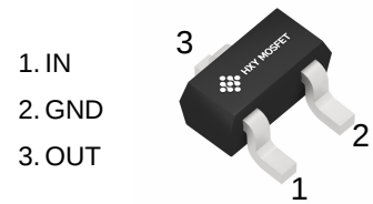
SOT-523 (SOT-523-3)
