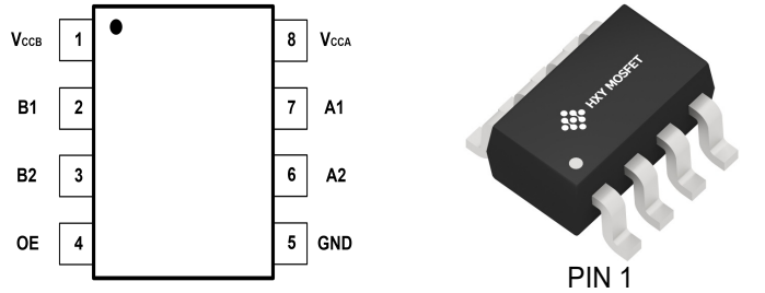
RS0102YH8 (SOT-23-8L) Package
