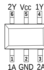
SOT-23-6L/SC-70-6
