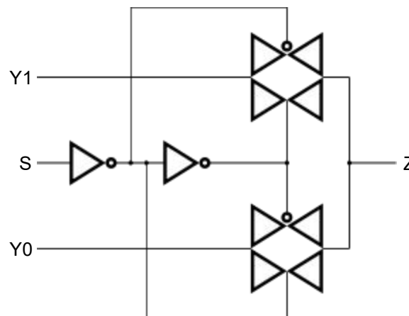
Figure 2. Logic diagram
