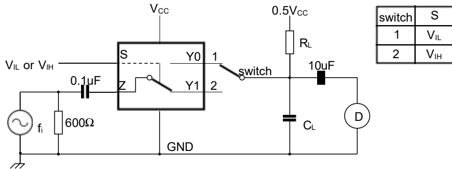
Figure 16. Test circuit for measuring total harmonic distortion
