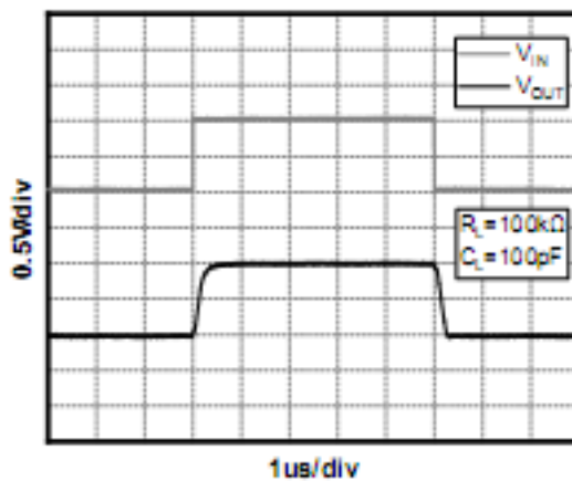
Figure 9. Large-Signal Step Response( V_S=1.5V )
