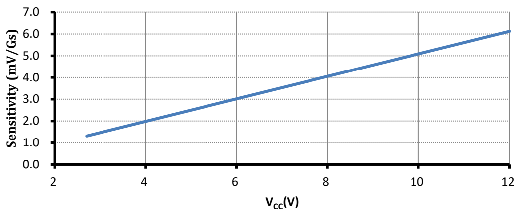
Sensitivity VS V_{CC} @25 °C
