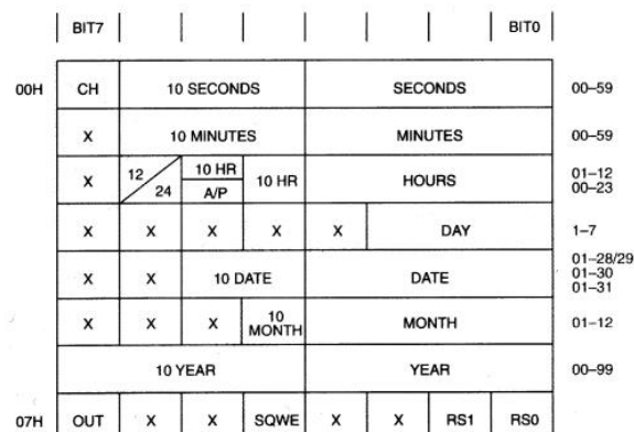
DS1307ZN+T&R TIMEKEEPER REGISTERS Figure 3
