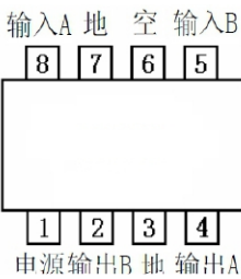
SOP-8
