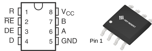
SOP-8(SOIC-8)
