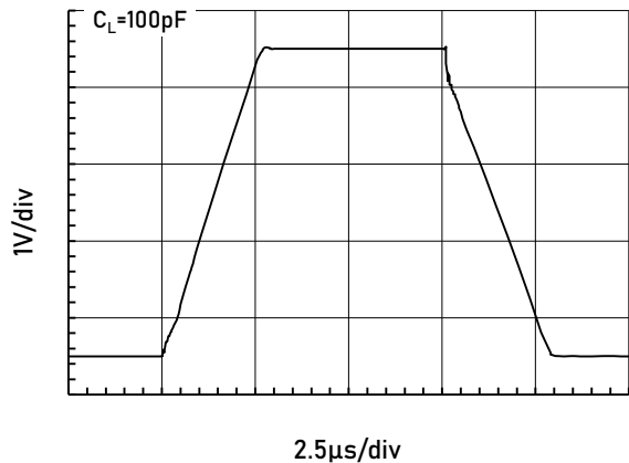
Large Signal Step Response (4V Step).
