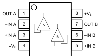
SOP-8
