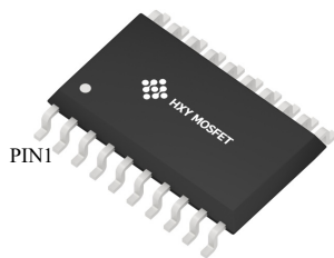
SOP-20(SOIC-20-300mil)
