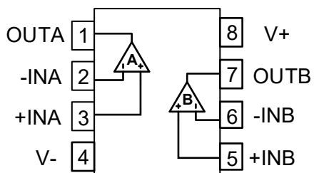
MSOP-8
