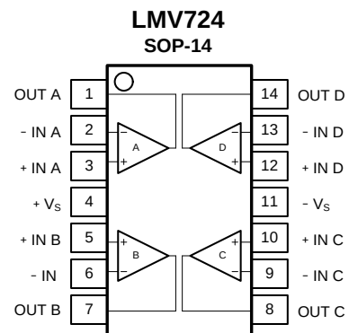
SOP-14
