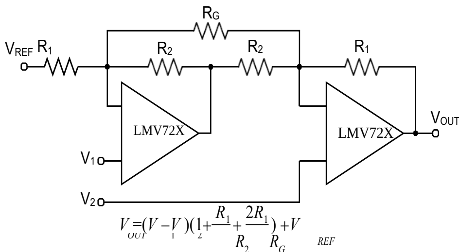
Fig. 17 Instrumentation Amplifier
