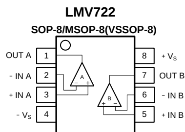
Figure 1. Pin Assignment Diagram
