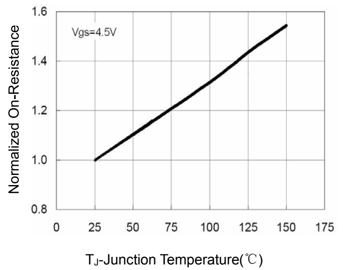
Figure 8 Drain-Source On-Resistance
