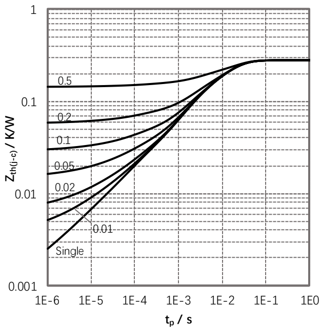
Fig 25. Transient Thermal Impedance
