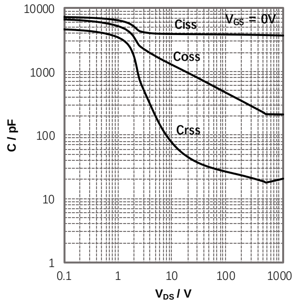
Fig 15. Capacitance Characteristics
