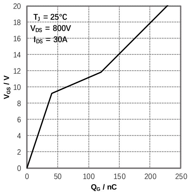
Fig 17. Gate Charge Characteristics
