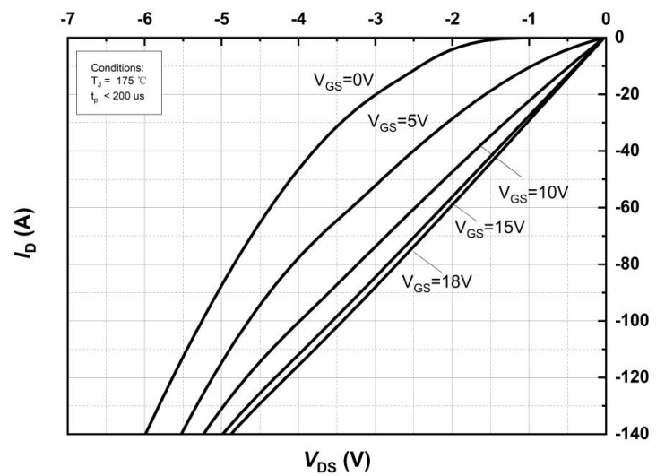
Figure 12. 3rd Quadrant Characteristic at T_j=175\text{°C}
