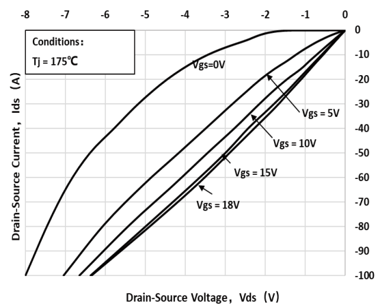
Fig 14: 3rd Quadrant Characteristic( T_J=175^{\circ}\text{C} )
