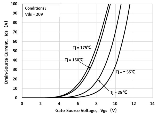
Fig 6: Transfer Characteristic
