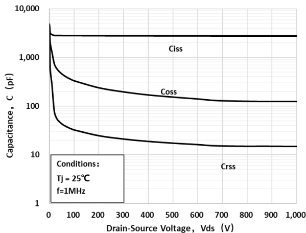
Fig 15: Capacitance Characteristic
