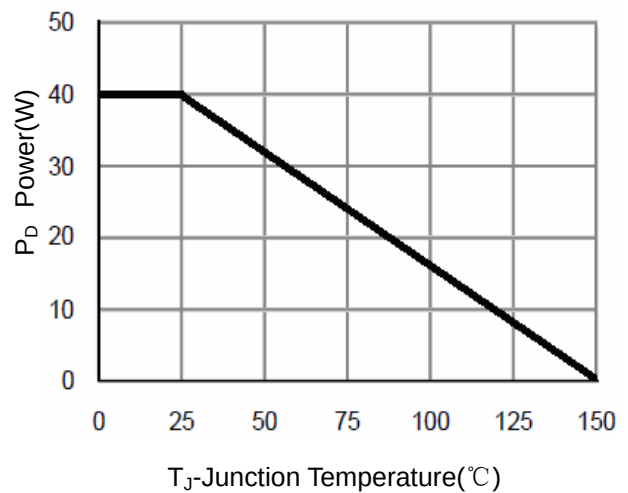
Figure 8 Power Dissipation
