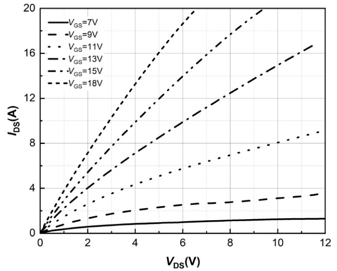
Figure 2 Output Characteristics
