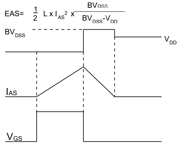
Fig. 8 EAS Waveform
