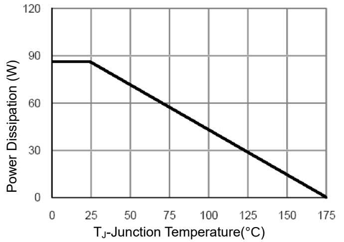
Figure 9 Power De-rating
