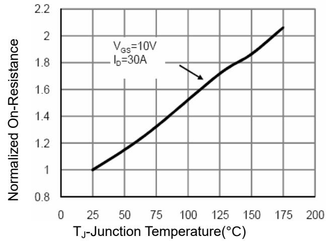
Figure 4 Rdson-Junction Temperature
