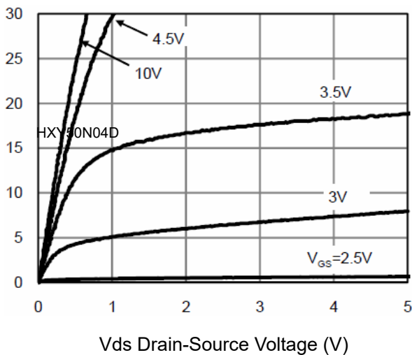
Figure 3 Output Characteristics
