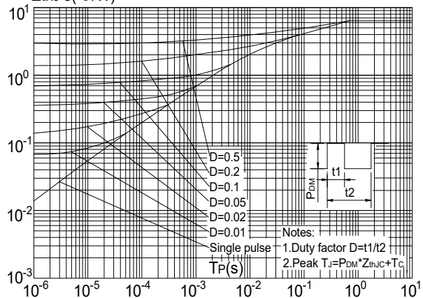
Figure.11: Maximum Effective Transient Thermal Impedance, Junction-to-Case Z_{thj-c} (^{\circ}\text{C}/\text{W})
