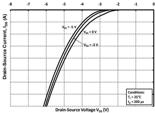
Figure 9. Body Diode Characteristic at 25\text{ }^{\circ}\text{C}
