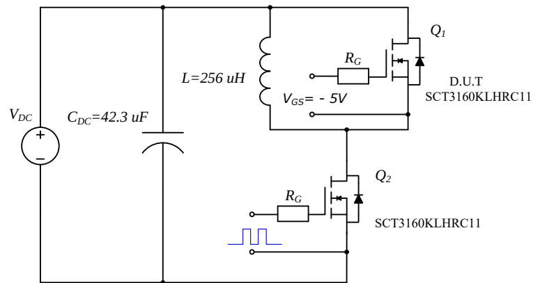
Figure 30. Clamped Inductive Switching Waveform Test Circuit
