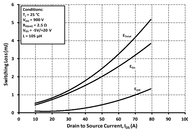
Figure 23. Clamped Inductive Switching Energy vs. Drain Current (V = 900V)
