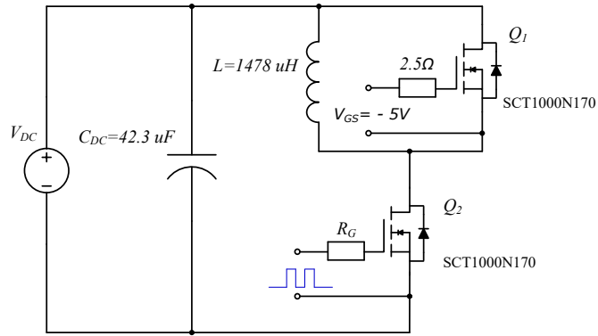
Figure 29. Clamped Inductive Switching Waveform Test Circuit
