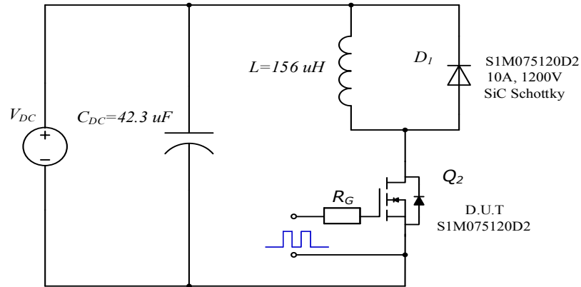
Figure 30. Clamped Inductive Switching Waveform Test Circuit
