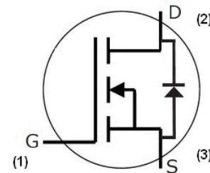
TO-247
