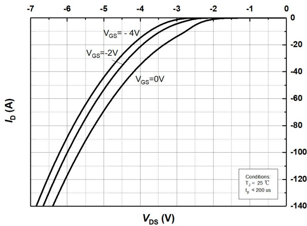
Figure 7. Body Diode Characteristics at T_j=25\text{ °C}
