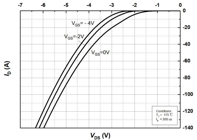
Figure 8. Body Diode Characteristics at T_j=175\text{ °C}
