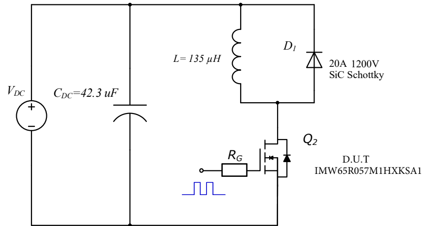
Figure 27. Clamped Inductive Switching Waveform Test Circuit
