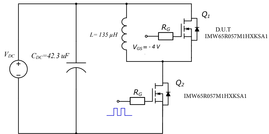
Figure 28. Body Diode Recovery Test Circuit
