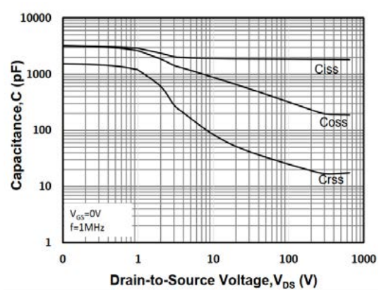
Fig 12: Capacitance Characteristics
