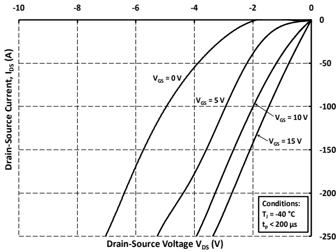
Figure 13. 3rd Quadrant Characteristic at -40 °C
