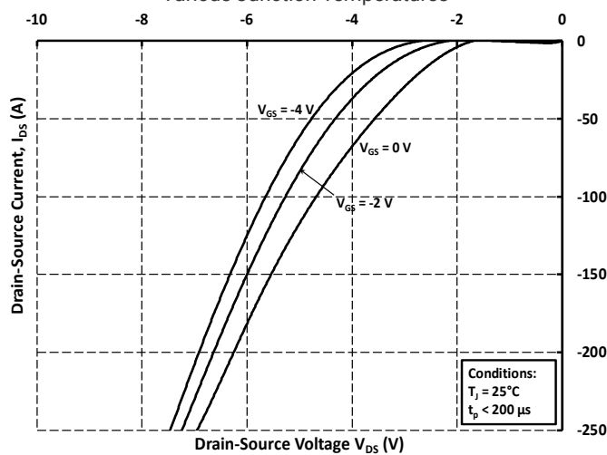
Figure 9. Body Diode Characteristic at 25^\circ\text{C}
