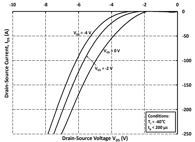
Figure 8. Body Diode Characteristic at -40^\circ\text{C}
