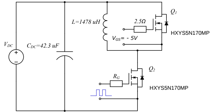
Figure 29. Clamped Inductive Switching Waveform Test Circuit
