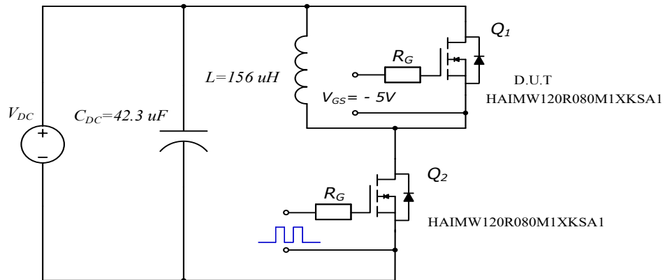
Figure 31. Body Diode Recovery Test Circuit
