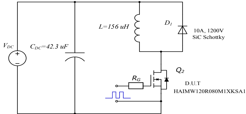
Figure 30. Clamped Inductive Switching Waveform Test Circuit
