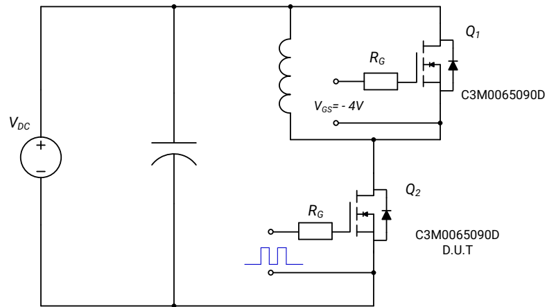
Figure 30. Clamped Inductive Switching Waveform Test Circuit
