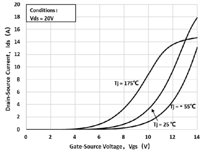
Fig 6: Transfer Characteristics
