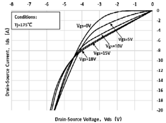
Fig 14: 3rd Quadrant Characteristics ( T_J=175^\circ\text{C} )
