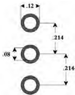
TO-247
