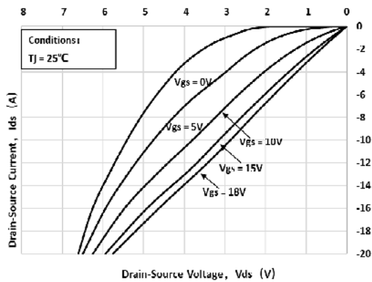
Fig 13: 3rd Quadrant Characteristics ( T_J=25^\circ\text{C} )
