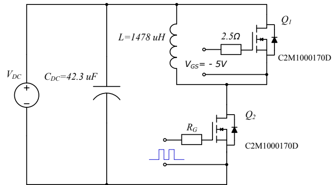
Figure 29. Clamped Inductive Switching Waveform Test Circuit
