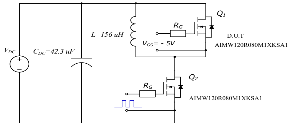
Figure 31. Body Diode Recovery Test Circuit
