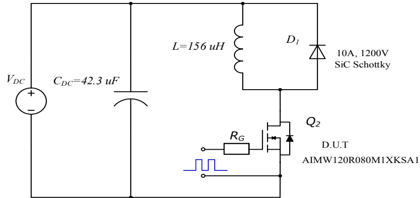
Figure 30. Clamped Inductive Switching Waveform Test Circuit
