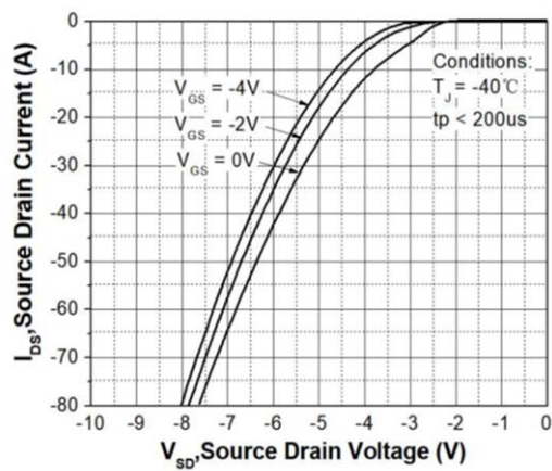
Fig 7: Body-diode Characteristic ( T_J = -40^{\circ}\text{C} )
