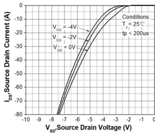
Fig 8: Body-diode Characteristic ( T_J = 25^{\circ}\text{C} )
