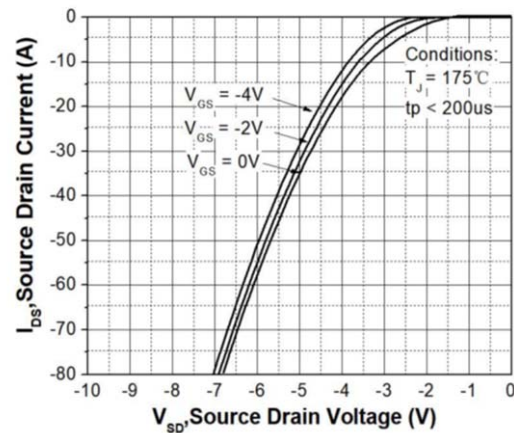
Fig 9: Body-diode Characteristic ( T_J = 175^{\circ}\text{C} )
