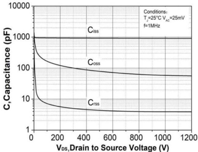
Fig 15: Capacitance Characteristic
