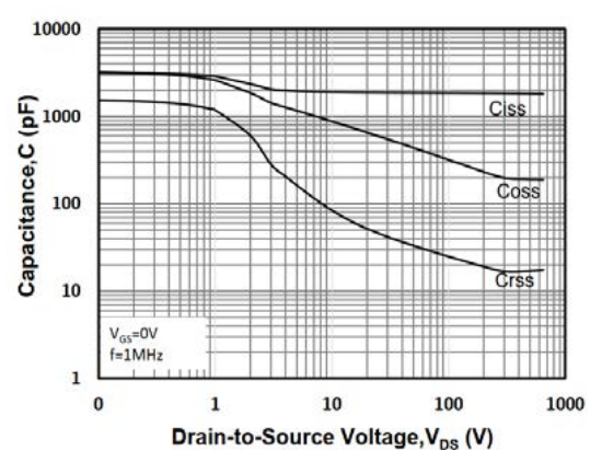
Fig 12: Capacitance Characteristics
