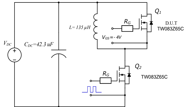
Figure 28. Body Diode Recovery Test Circuit
