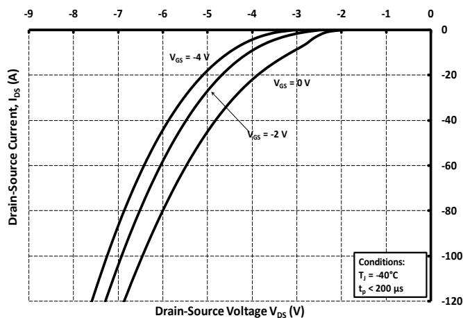
Figure 8. Body Diode Characteristic at -40\text{ }^{\circ}\text{C}
