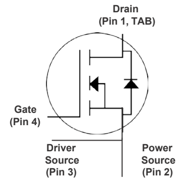
TO-247H-4L (TO-247H-4)
