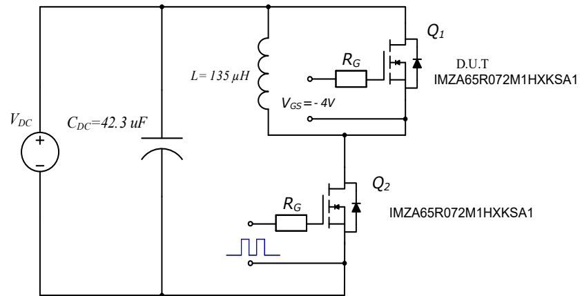
Figure 28. Body Diode Recovery Test Circuit
