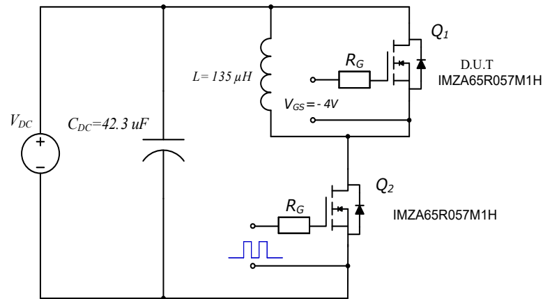
Figure 28. Body Diode Recovery Test Circuit
